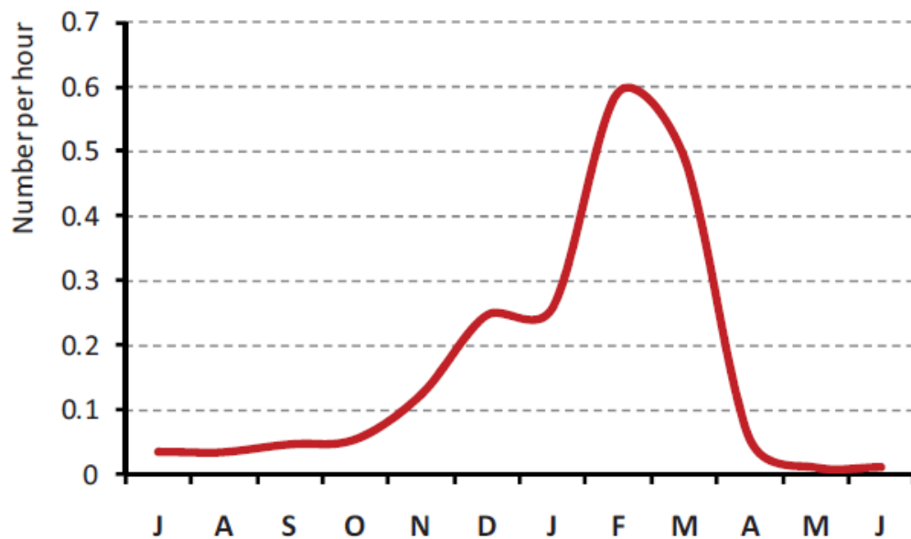
Figuur 7.9 Seasonal pattern in numbers of Harbour Porpoises per hour of observation during seawatching (n/h), mainland coast observatories only (Scheveningen – Huisduinen, 1990-2010; from Camphuysen 2011).
