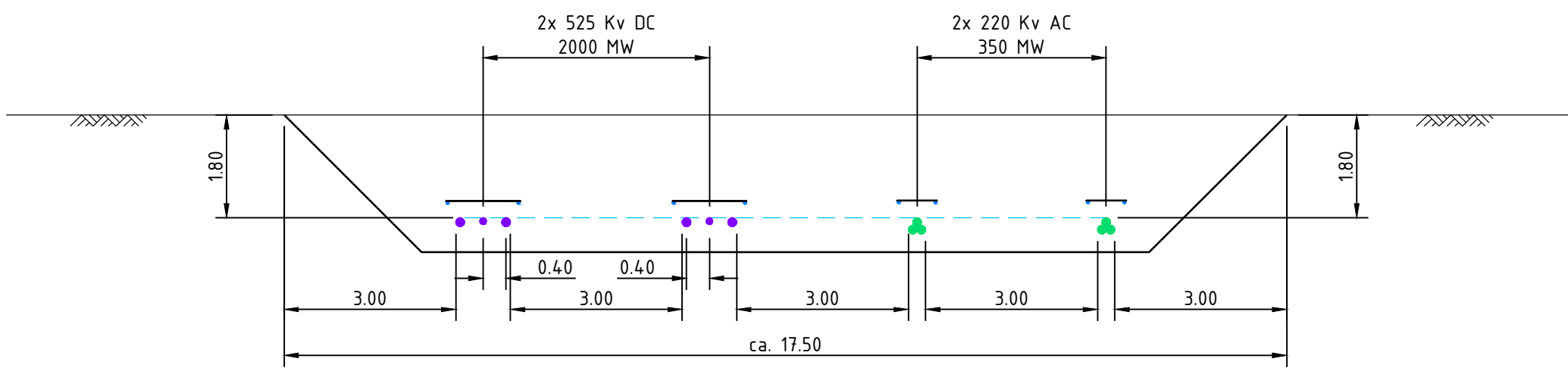
CROSS SECTION 1 – 4.7 GW; OPEN EXCAVATION SCHAAL 1:100
