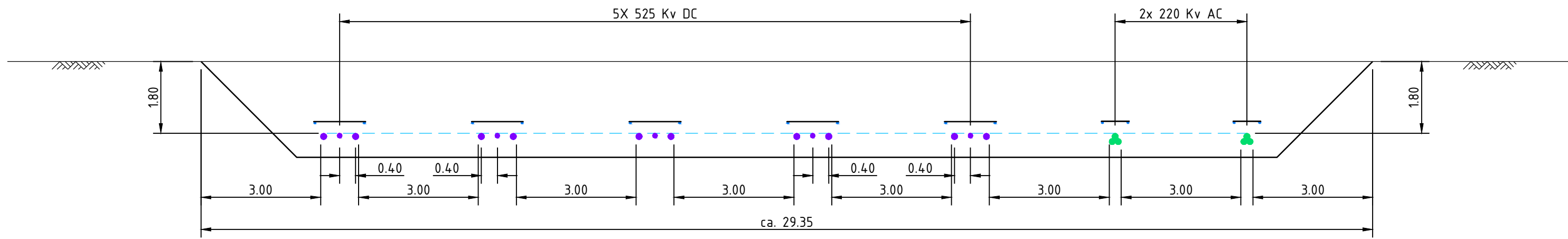
CROSS SECTION 1 – 10.7 GW; OPEN EXCAVATION SCHAAL 1:100
