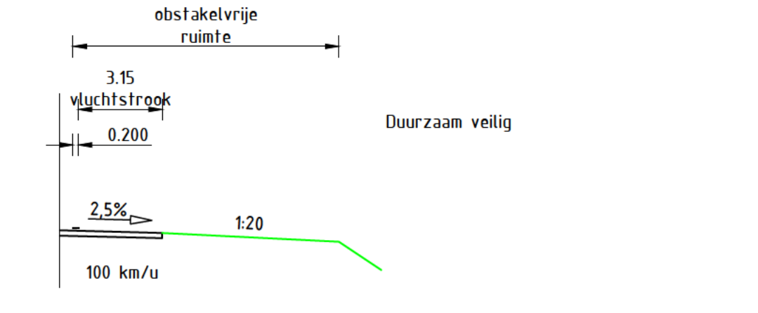
Principeprofiel 2: obstakelvrije buitenberm
