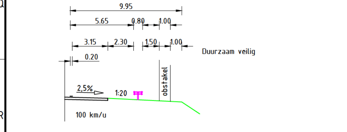
Principeprofiel 1: obstakel in buitenberm
