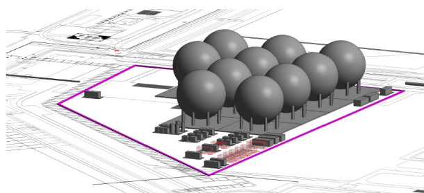
Figuur 2.5 3D-impressie van de terminal storage and pumping
